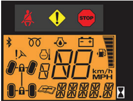
Digital instrument display (fuel not on 560E models)
