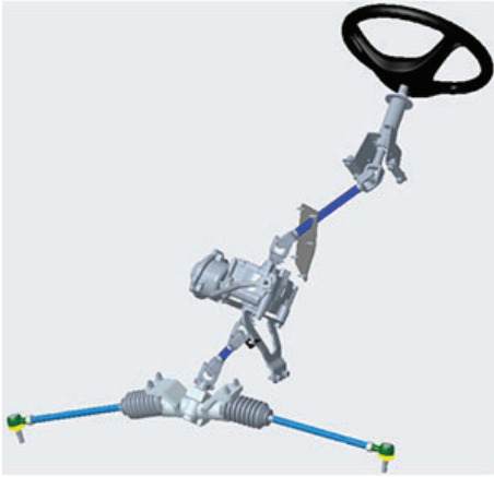
XUV590M with power steering
